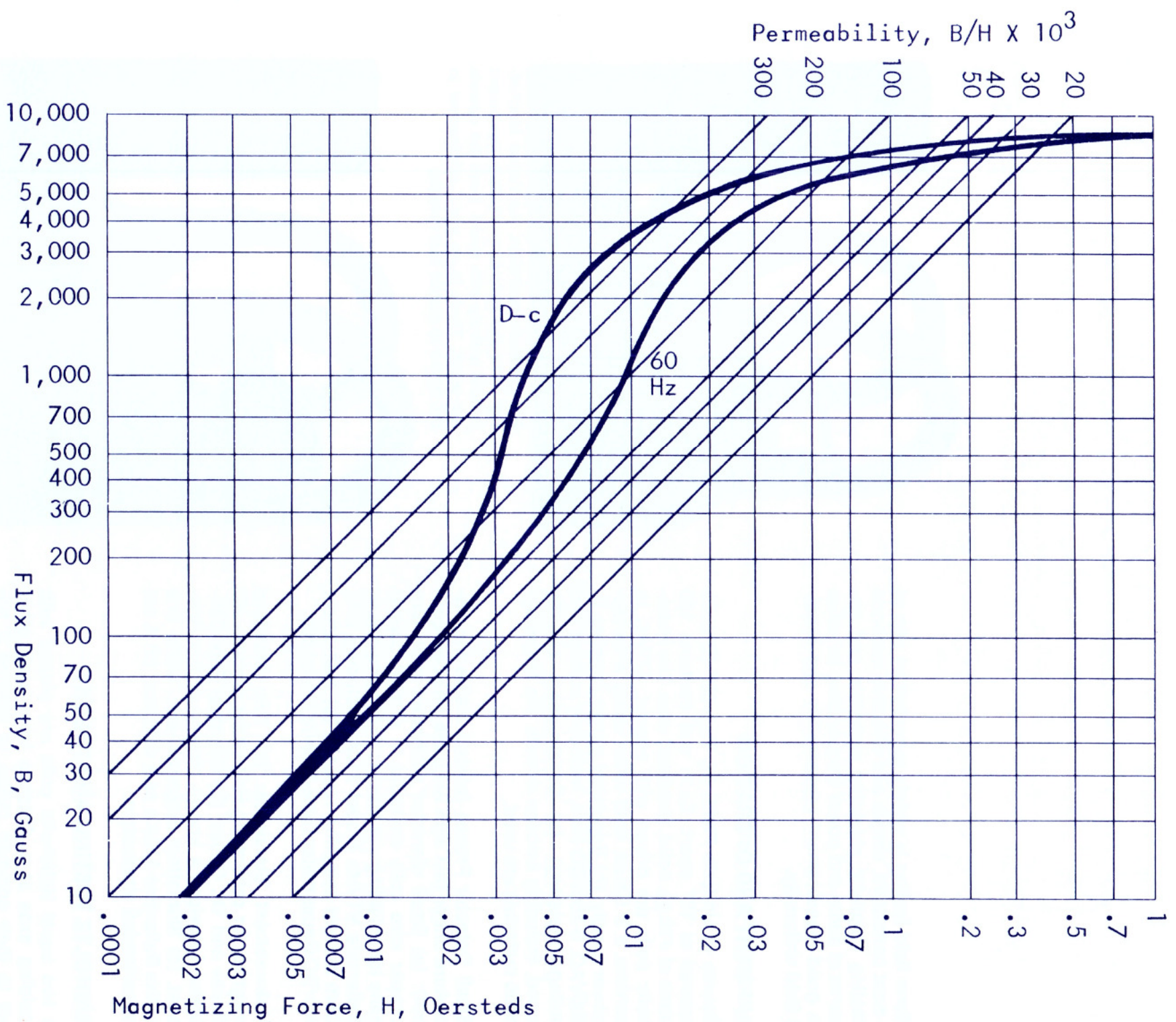
Typical magnetization curves of AD-MU-80 (.014 thickness).
